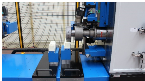
Fig. 1 – 2 Horizontal Trimming-Beading Machine R400-I for tubes 300 – 2000 mm length
